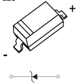
SOD-123
