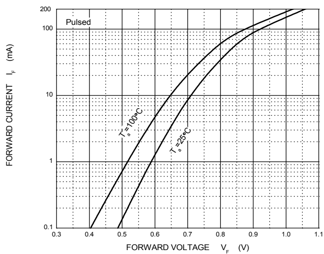
Forward Characteristics
