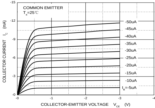
Static Characteristic
